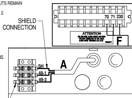
DETAIL 2 HEAT REJECTION INTERLOCK (F)
