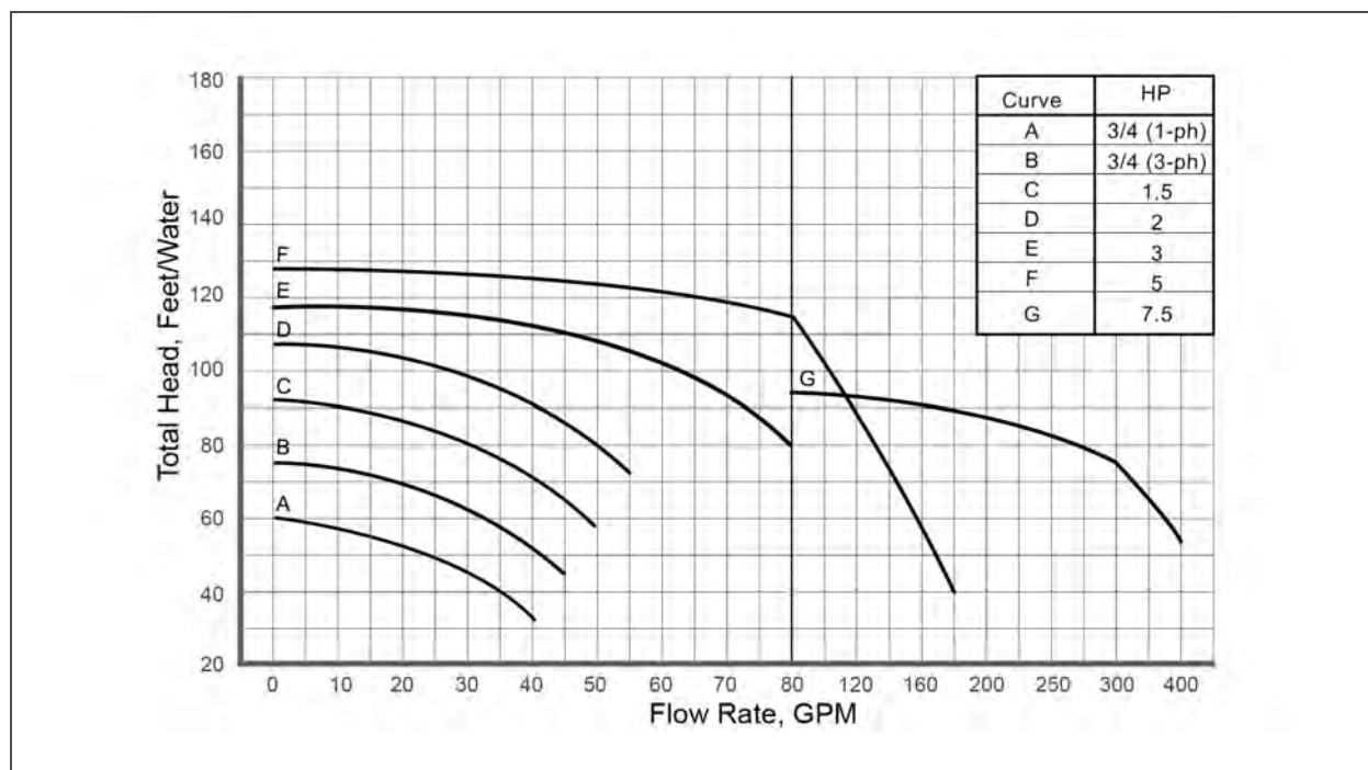
Figure 8.1 Pump curve, 60 Hz
